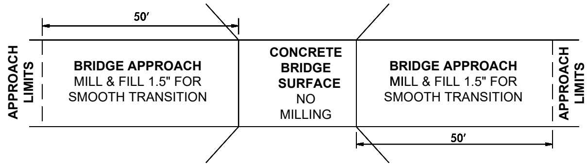
DETAIL FOR MAP # 1 & 2 / STRUCTURE # # 0015 & #0028
