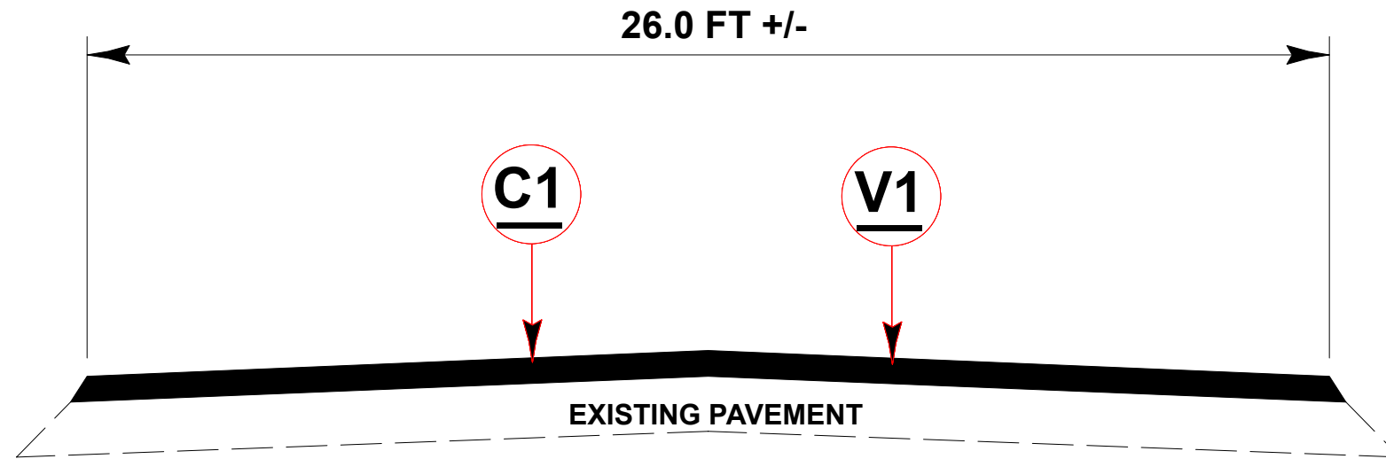
TYPICAL SECTION # 1 MAP(S) # 1 & 2
